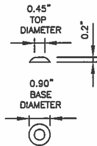
RAISED TRUNCATED DOME PATTERN
