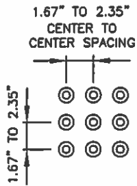
RAISED TRUNCATED DOME PATTERN
